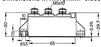
Dimensions in mm (1mm=0.0394")
